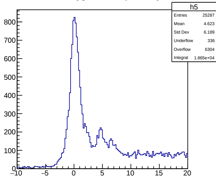
Exd {tgtc<8.0&&pidf==2}
