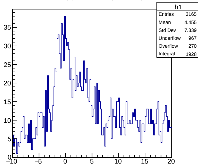
Ext {tgtc<8.0&&pidf==3}
