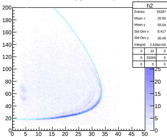
Etot:ThetaLab {tgtc<8.0&&pidf==2}
