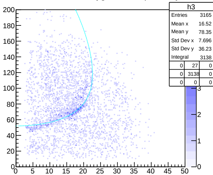
Etot:ThetaLab {tgtc<8.0&&pidf==3}
