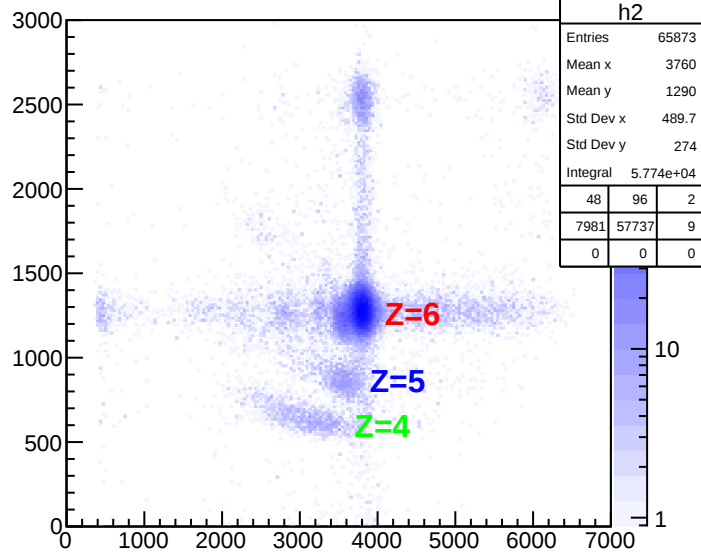
ICNumexo.Energy:PLASTIC_Q {pdf[4]==4}
