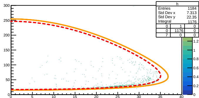
ELab:Theta3
