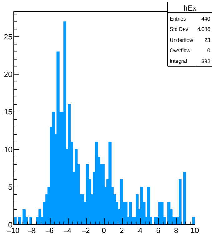
Ex {TelescopeNumber==1}
