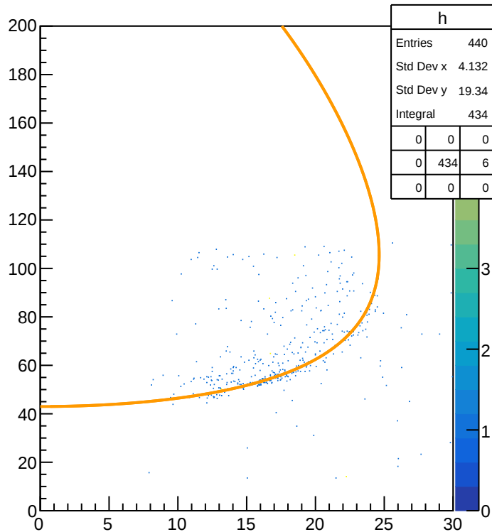
ELab:Theta3 {TelescopeNumber==1}
