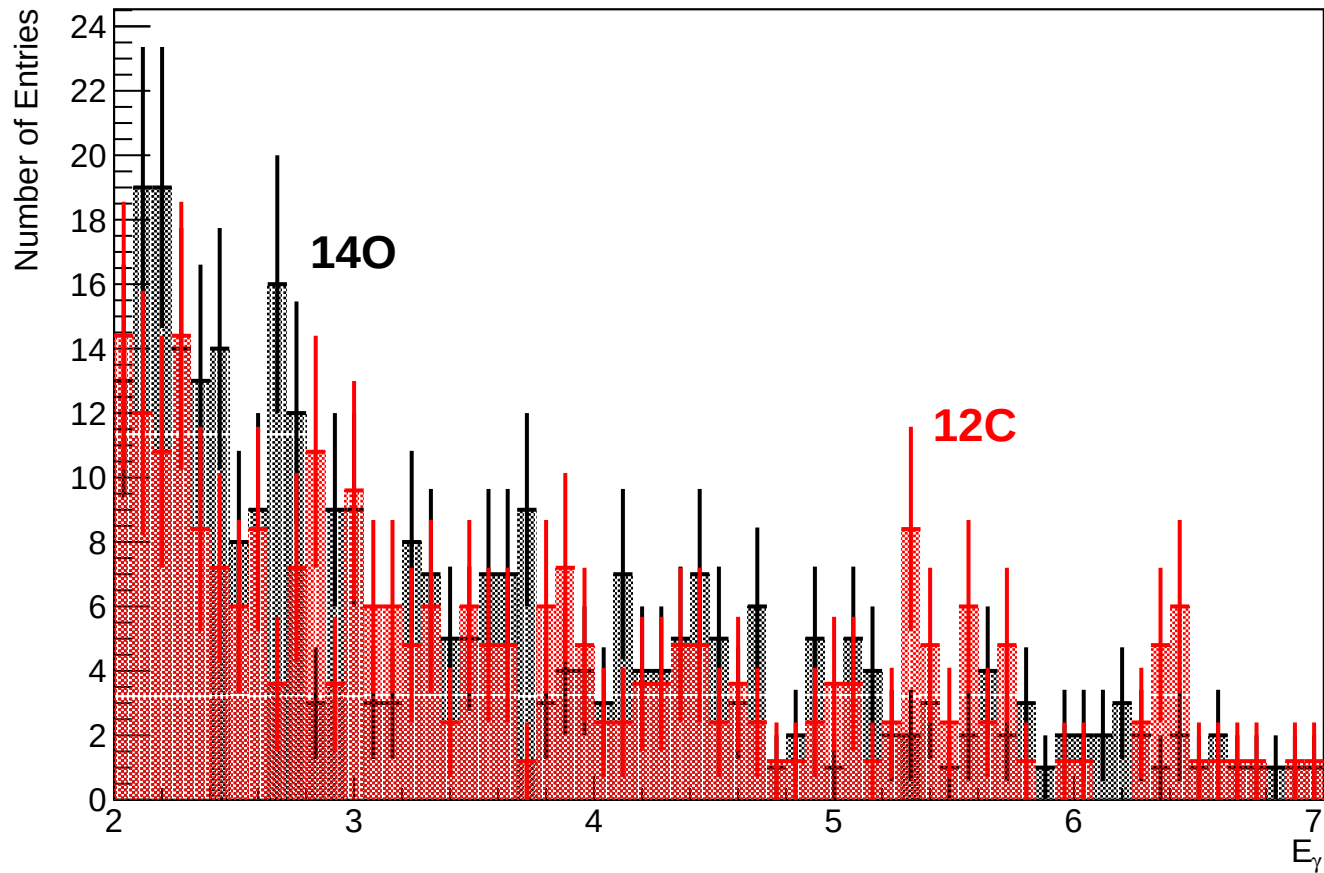
EXL prompt energy with DeE/ToF conditions on protons
