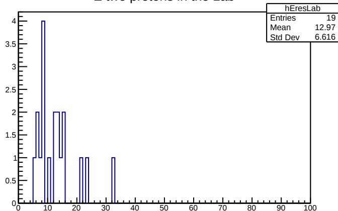
E two protons in the Lab
