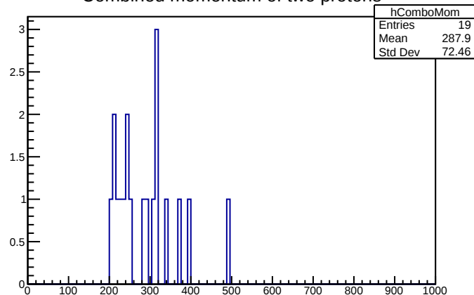
Combined momentum of two protons
