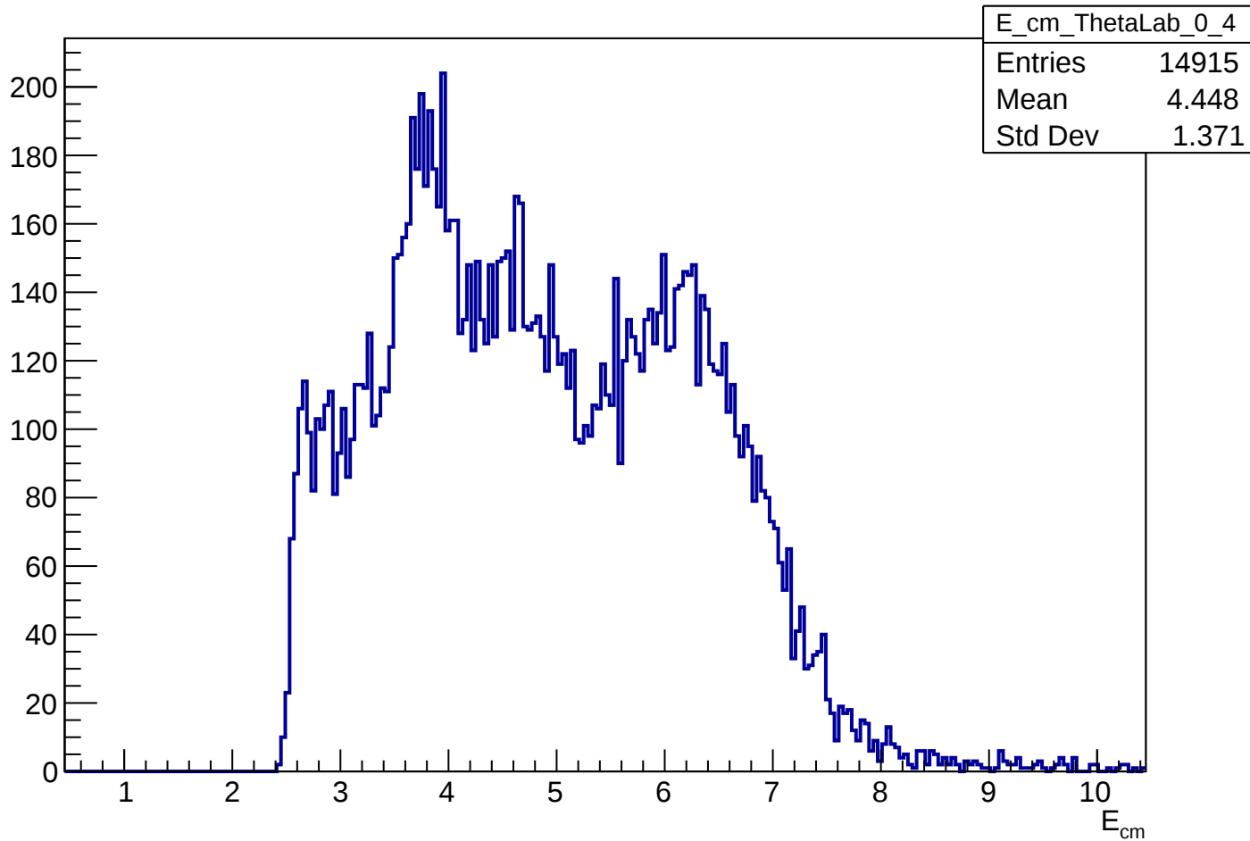
histogram E cm vs ThetaLab 14N(p,p)14N
