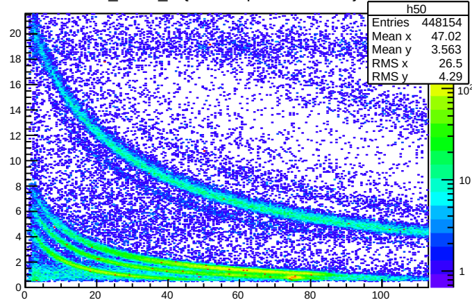
Si_E:Csl_E {TelescopeNumber==1}
