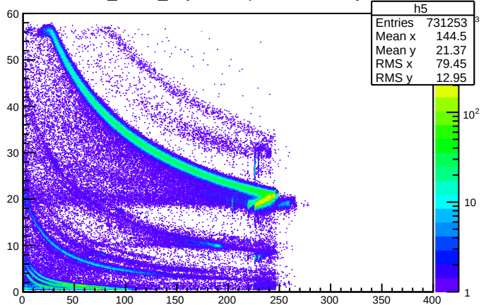
Si_E:Csl_E {TelescopeNumber==4}
