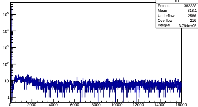
T_PL_CHIO
