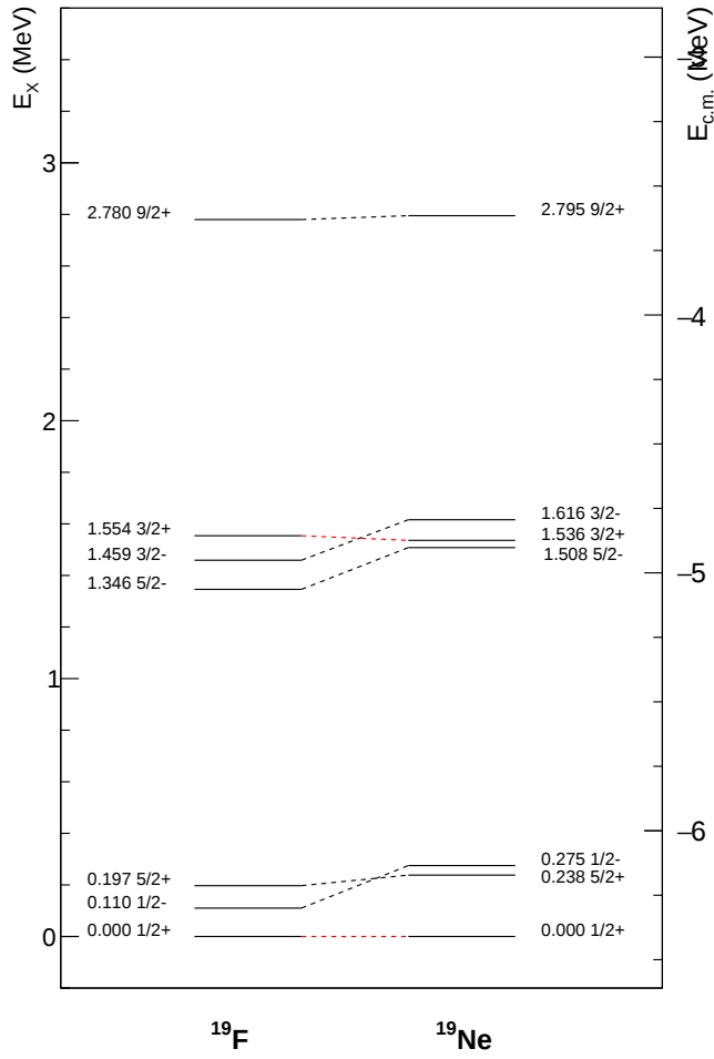
FIG. 1. Level scheme of ^{19}\text{Ne} nucleus up to E_x = 3.6 MeV and comparison with its mirror nucleus ^{19}\text{F} . Mirror pairs are linked with dashed lines. Red colour indicates mirror connection for \ell = 0 states.
