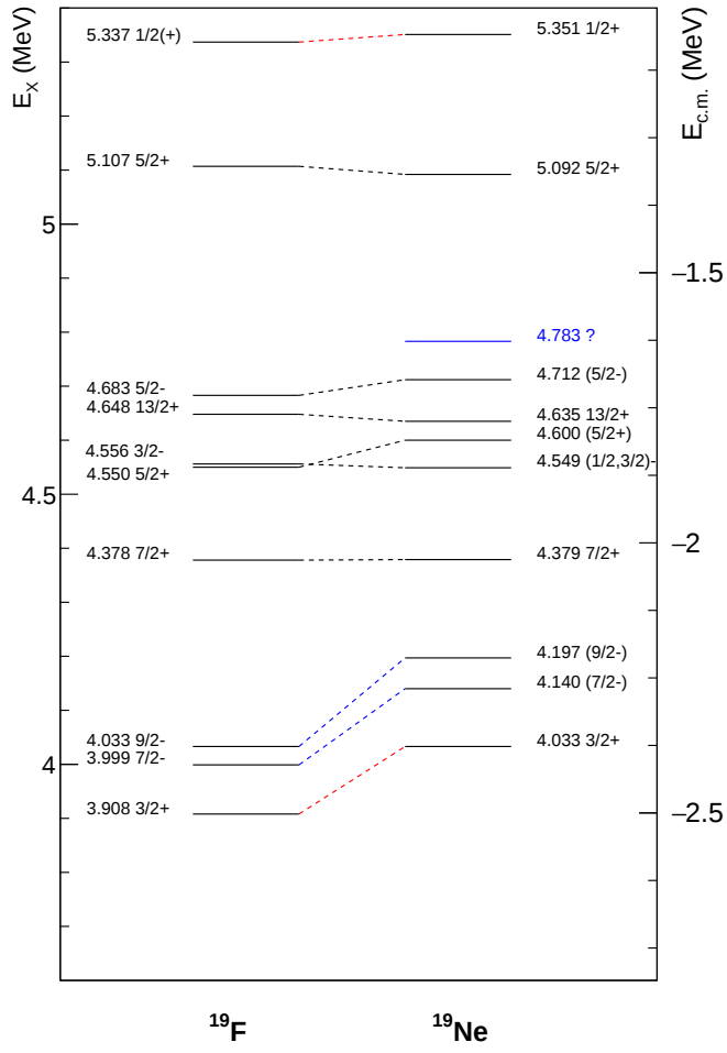
FIG. 2. Same as Fig. 1 for 3.6 \text{ MeV} < E_x < 5.4 \text{ MeV} . Information in blue is discussed in Sec. IA 1.
